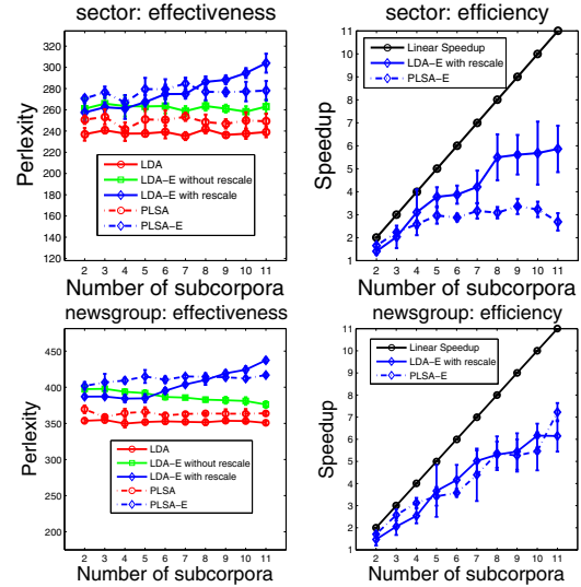
Figure 5. Results with varying number of subcorpora.
