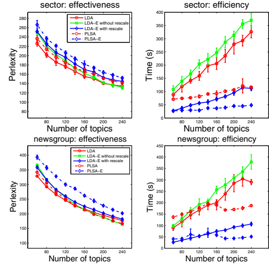
Figure 4. Results with varying number of topics.
