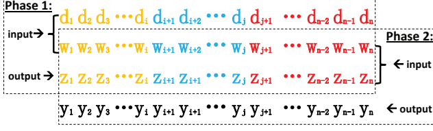
Figure 2. Illustration of Gibbs Sampling
